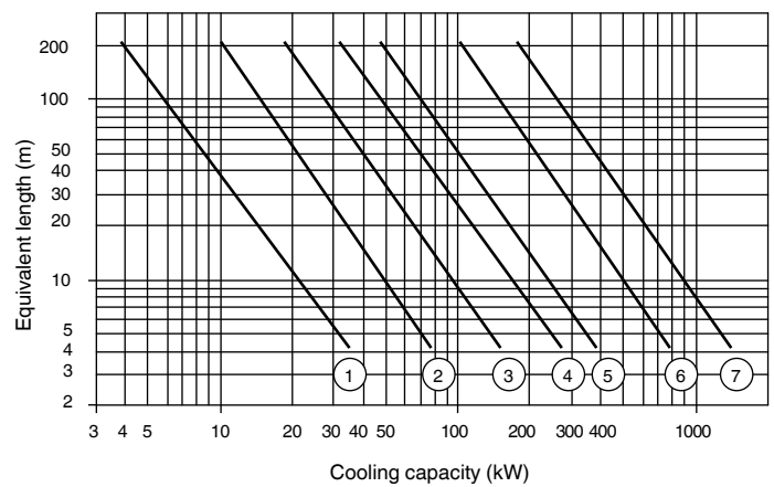
Liquid piping
